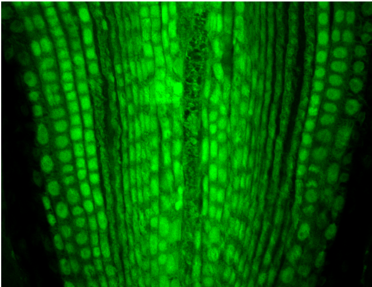
Front cover: Alisma plantago-aquatica L., a longitudinal section of the apical part of a root showing schizogenous aerenchyma (see the article by Ovcharenko & Shevchenko on pages 197–205 in this issue).
